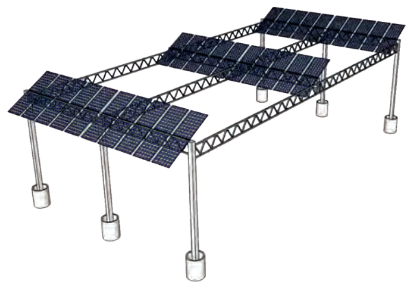
Fig. 52: Illustration of different system types oriented east-west, south and south-east © Fraunhofer ISE
