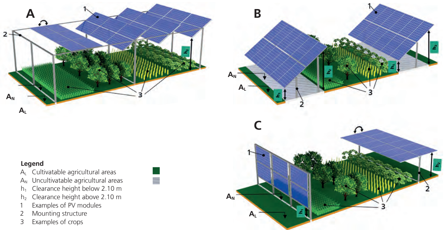
Fig. 10: Illustration of the categories and forms of land use as set out in DIN SPEC 91434 © Fraunhofer ISE
