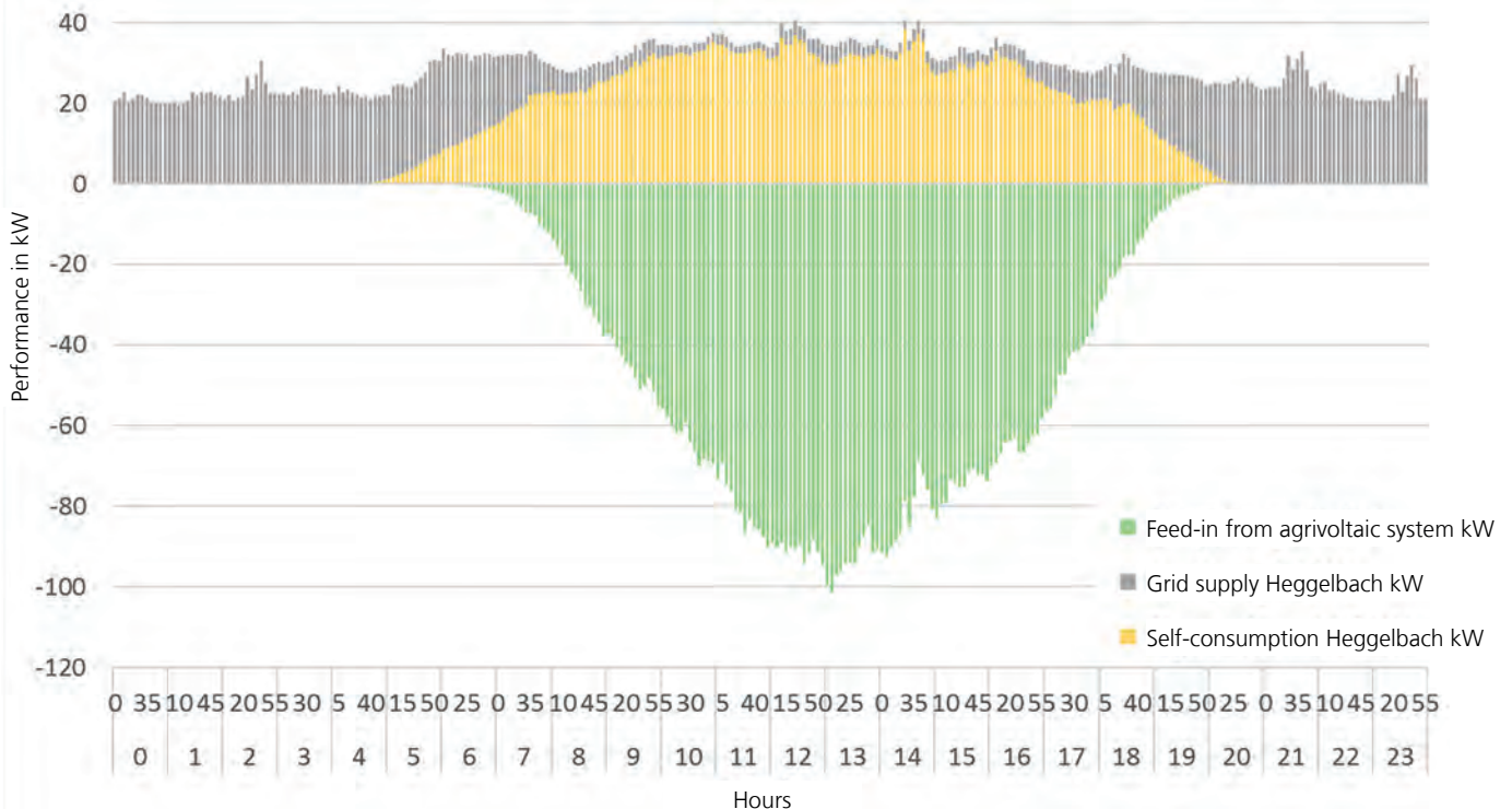
Fig. 14: The agrivoltaic system at Hofgemeinschaft Heggelbach enabled the farm to cover almost all of its energy demand in summer 2017 using the power generated with the system © BayWa r.e.
